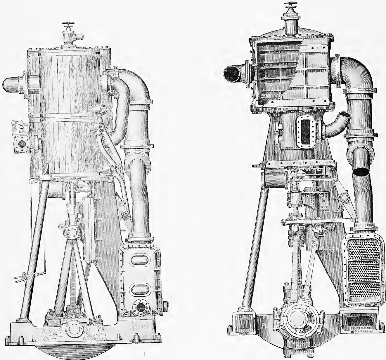
WELLS' PATENT BALANCED ENGINE.
